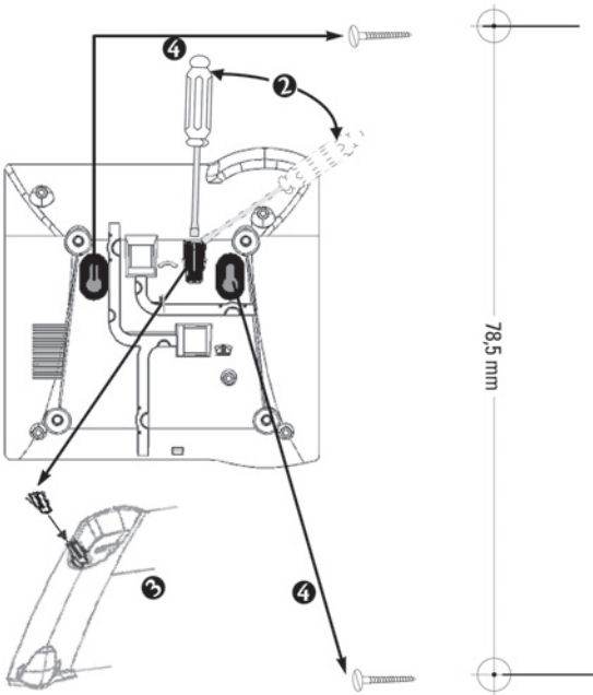
Wall mounting diagram
